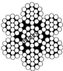
wire rope (flexible 7x19) stainless steel, GY-201
