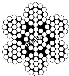
wire rope (flexible 7x19) stainless steel, GY-201
