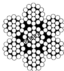
wire rope (flexible 7x19) stainless steel, GY-160
