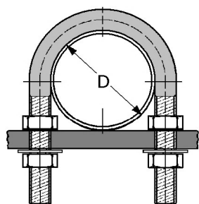
"U" pipe support stainless steel, GY-180
