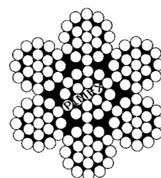
wire rope (flexible 7x19) stainless steel, GY-160
